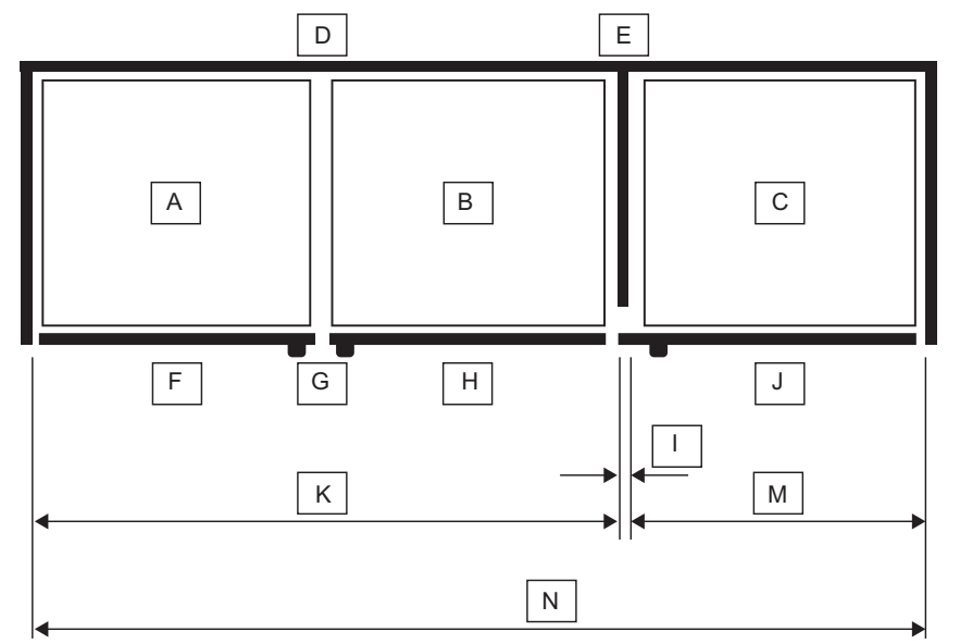
Diagram A – Smallest Cutout (Door Opening is Restricted) Applies to Custom Panels Only.
