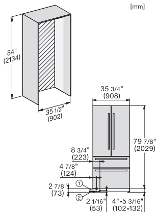
KFMC3846FD, MasterCool III, PACS, with stainless steel front, installation (US)
