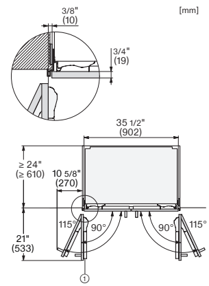
KFMC3846FD, MasterCool III, PACS, with stainless steel front, top view (US)
