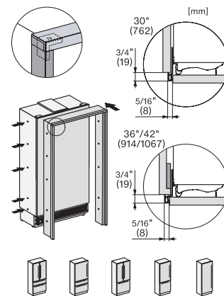
KFMC3632R+L, KFMC3642R+L, KFMC3836R+L, KFMC3834R+L, KFMC3858FD, MasterCool III, integration, neutral, installation
