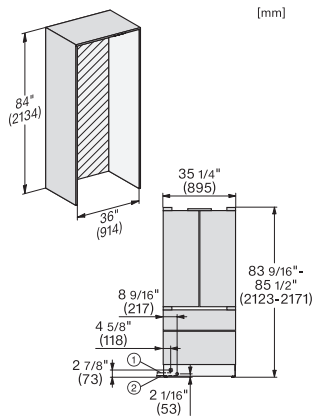
KFMC3846FD, MasterCool III, installation, panel ready (US)
