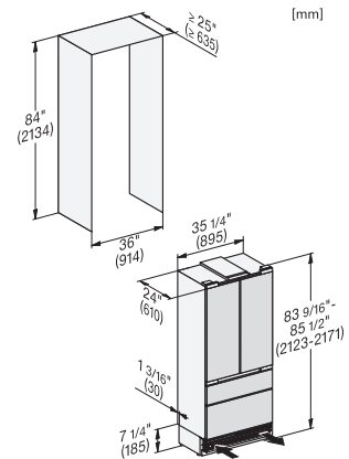
KFMC3846FD, MasterCool III, integration, panel ready (US)
