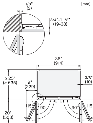
KFMC3846FD, MasterCool III, panel ready, top view (US)
