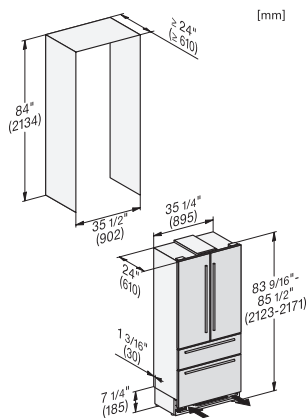
KFMC3846FD, MasterCool III, PACS, with stainless steel front, integration (US)
