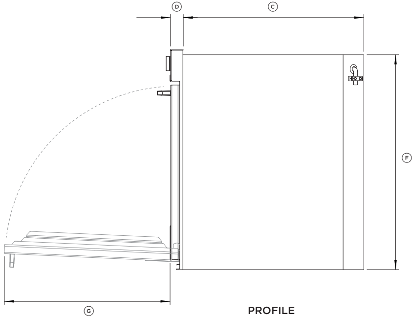
PROFILE
