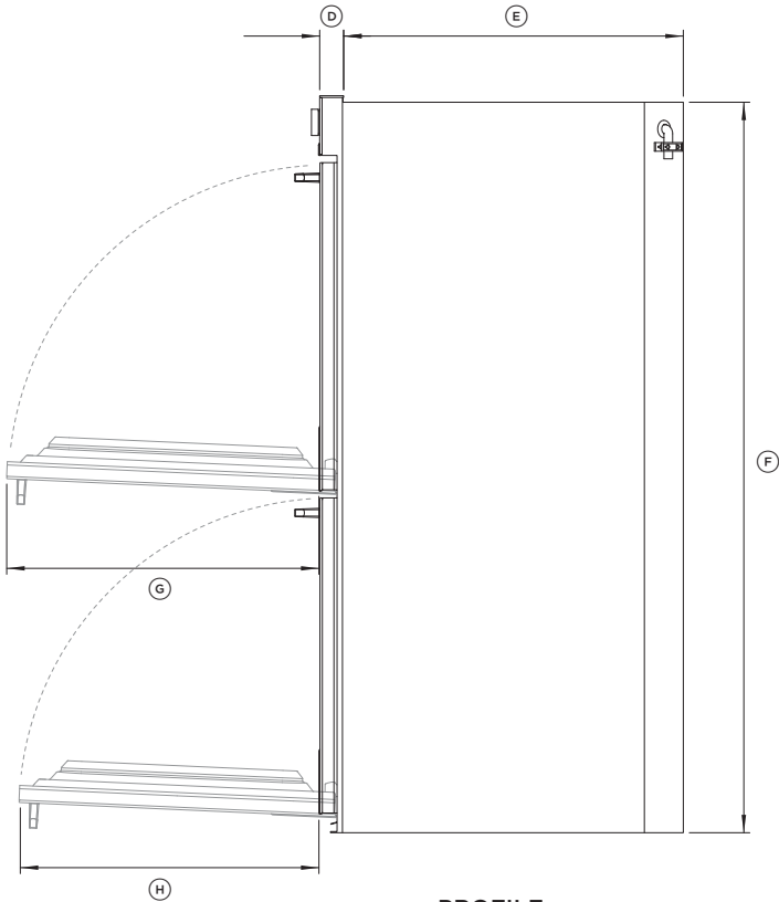
PROFILE
