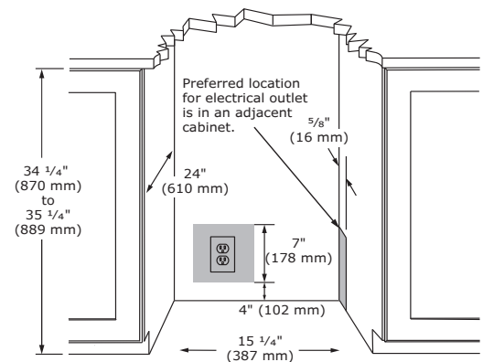
Cabinet Cut-Out
