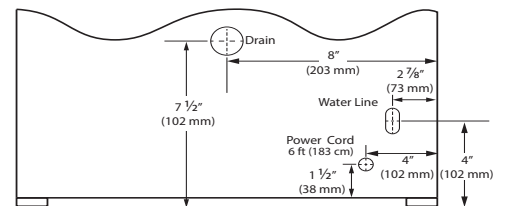
Cabinet Cut-Out
