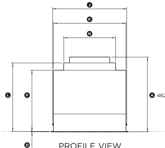
PROFILE VIEW
