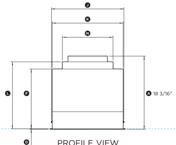
PROFILE VIEW
