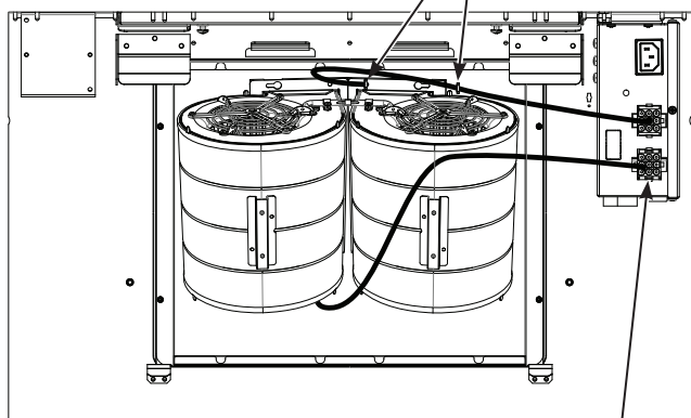
Motor Mating Connector Location
