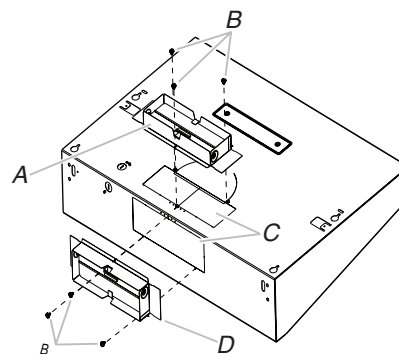
A. Vertical air transition B. 3.5 x 9.5 mm screws C. Vent knockouts D. Horizontal air transition
