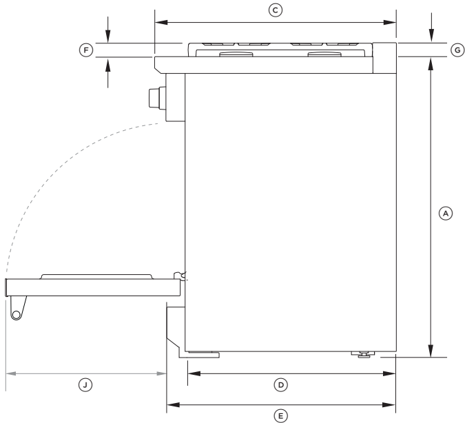
PROFILE
