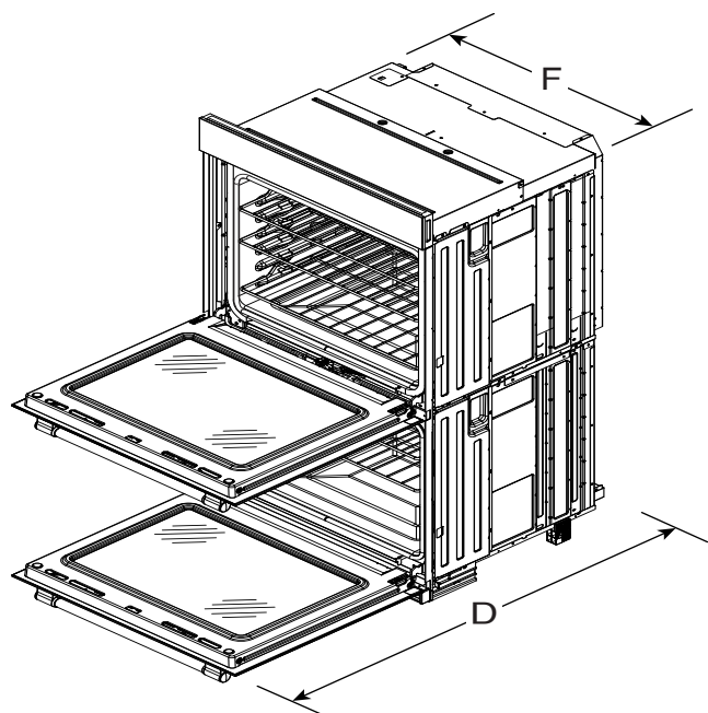
ANGLED VIEW
