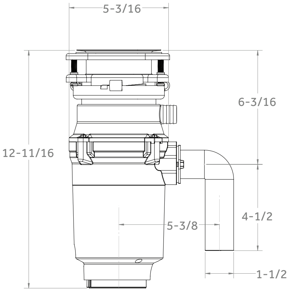
Disposall® Food Waste Disposer Dimensions (in Inches)
