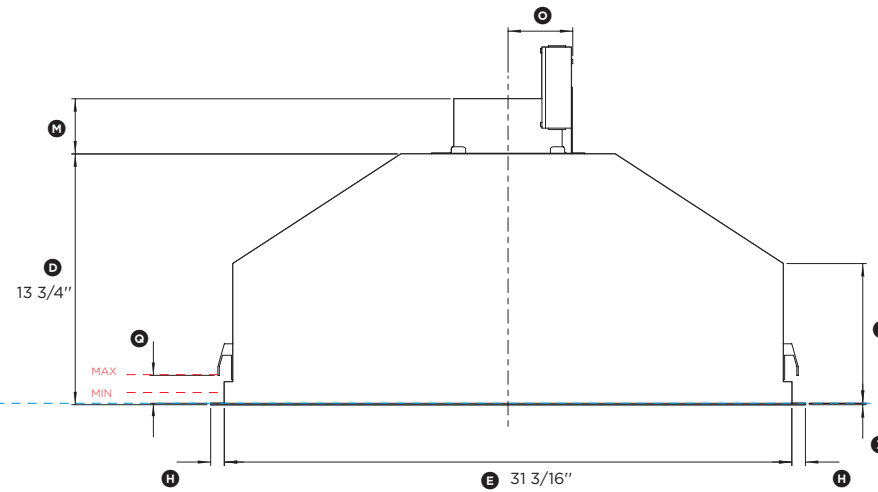
PROFILE VIEW
