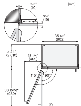
KFMC3642R, KFMC3642L, KFMC3844R, KFMC3844L, MasterCool III, PACS, with stainless steel front, top view
