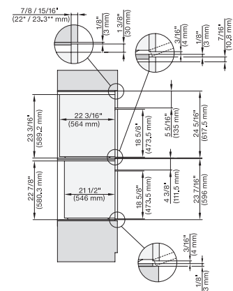
DGC7x8x(X)(+EBA7868), side view, 30 Zoll, Flush inset, combi, XXL, 650S
