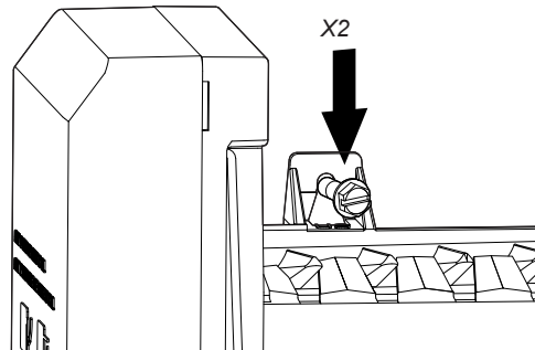
Mounting ice maker on top screws
