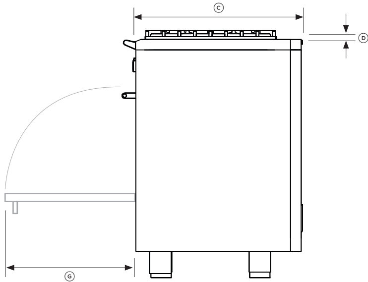
PROFILE
