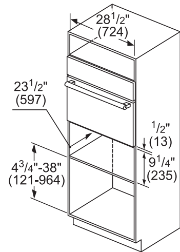
Standard Installation
