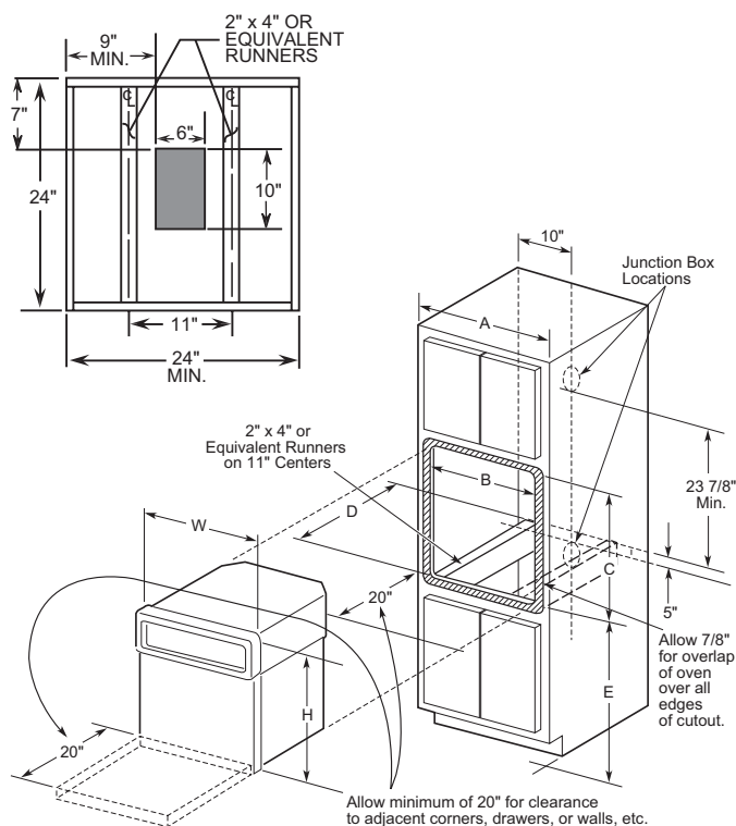
Fig. 1 — Single Oven
