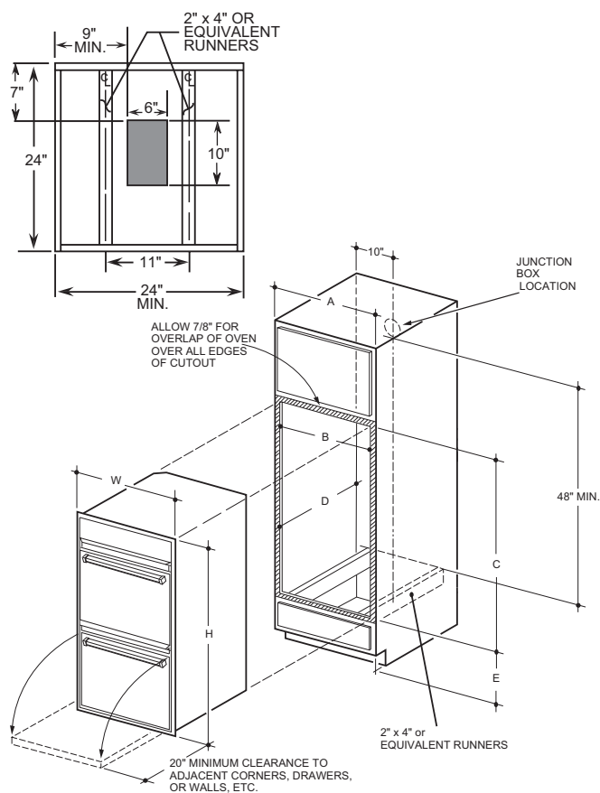
Fig. 2 — Double Oven
