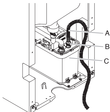
A. Drain Tube B. Clamp C. Drain Pump
