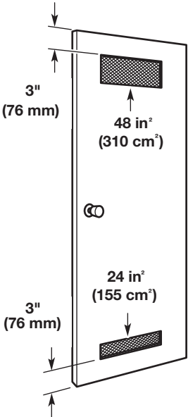
Closet Door Minimum Acceptable Vent Sizes
