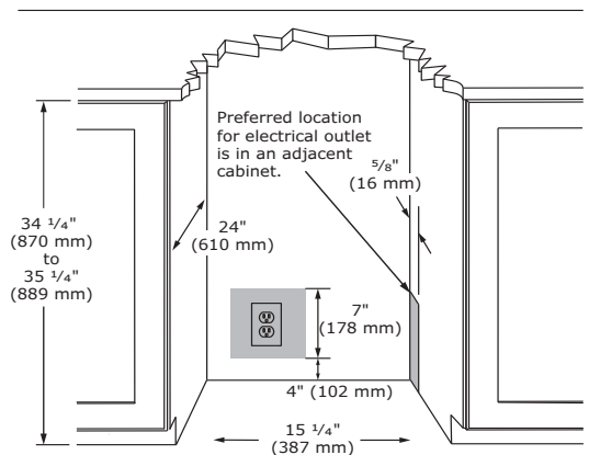
Cabinet Cut-Out
