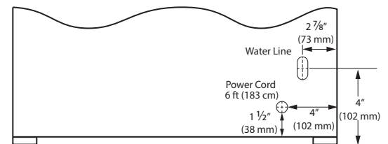
Cabinet Cut-Out
