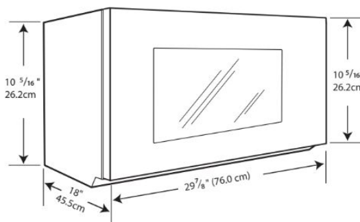
HS Horizontal
