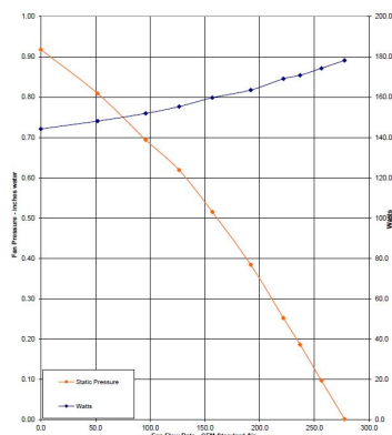
HS Vertical
