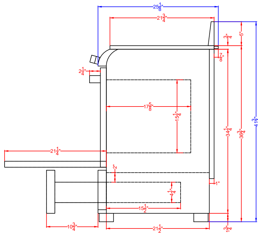
PROFILE VIEW
