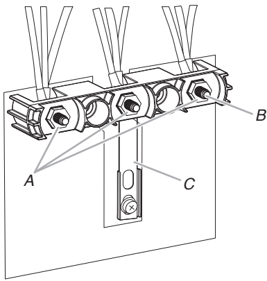
A. 10-32 hex nuts B. Terminal Posts C. Ground-link strap
