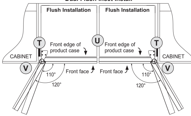
Dual Flush Inset Install
