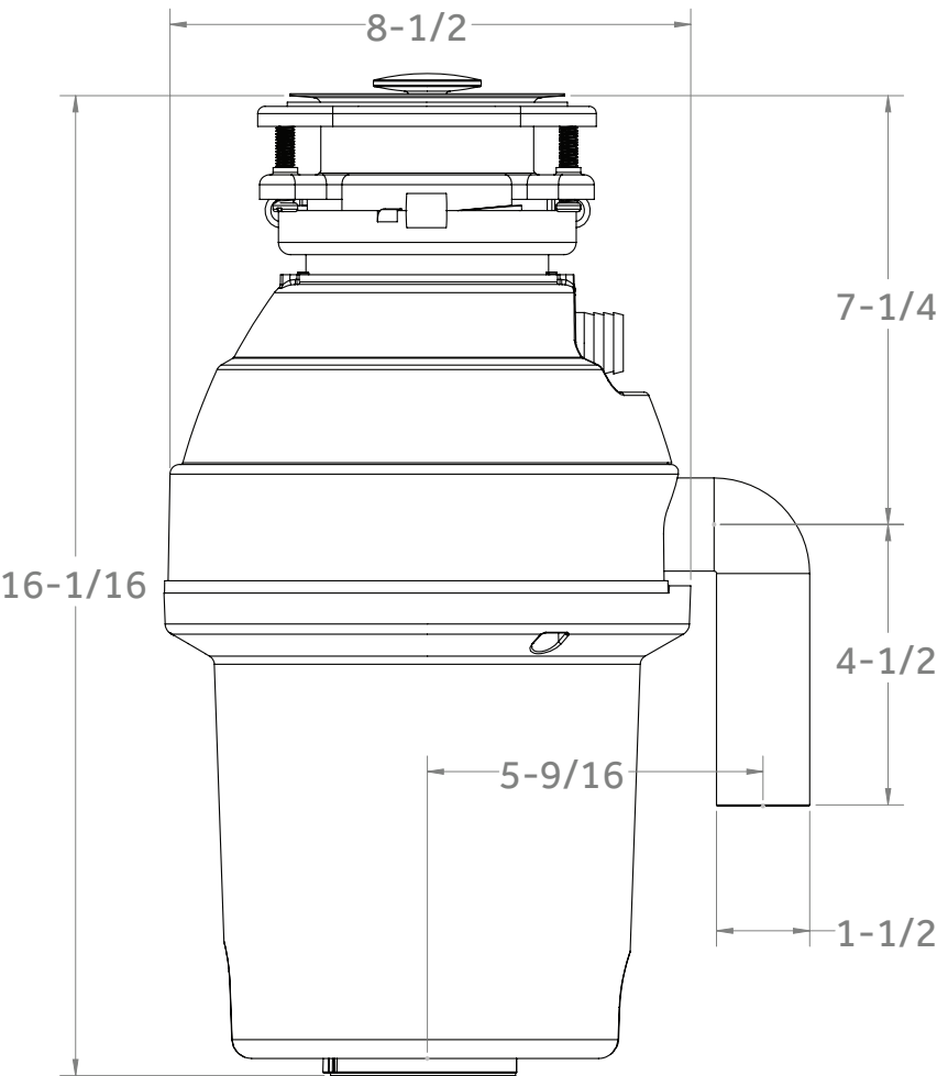
Disposall® Food Waste Disposer Dimensions (in Inches)
