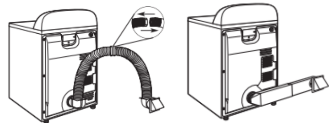
Over-The-Top installation (also available with one offset elbow) Periscope installation
