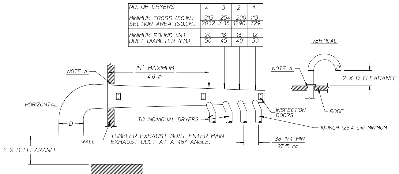
MULTIPLE DRYER VENTING (MAYTAG76 PC) WITH 8" (20.3 cm) DIAMETER (1200 CFM [34 cmm]) EXHAUST CONNECTIONS AT COMMON DUCT
