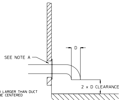
HORIZONTAL DUCTING
