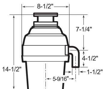
GFC720N
