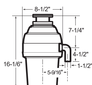
GFC1020N
