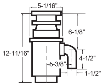
GFC520N GFC525N
