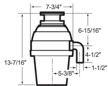
GFC530N GFC535N
