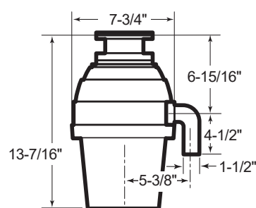
GFC530N GFC535N
