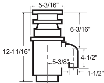
GFC320N GFC325N
