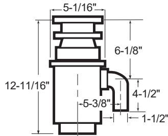
GFC520N GFC525N
