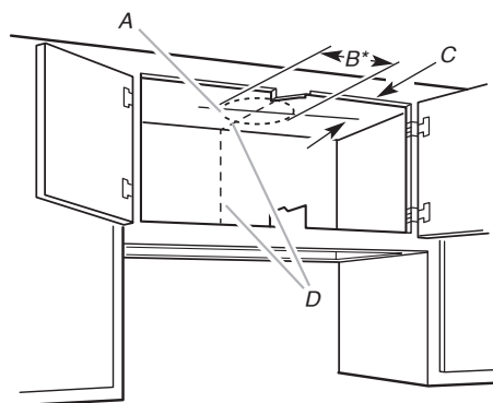
A. Cutout B. *See chart below. C. 7 \frac{3}{4} " (19.7 cm) centerline to cabinet front D. Centerline
