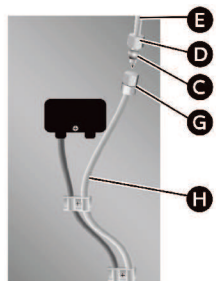
D 1/4" water line E 1/4" compression nut C Ferrule (sleeve) Brass G fitting H Water inlet
