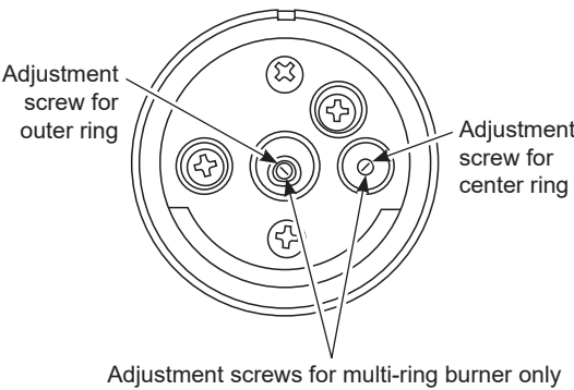
Adjustment screws for multi-ring burner only
