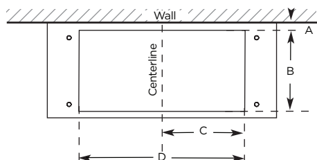
UPPERHOOD MOTOR HOUSING DIMENSIONS
