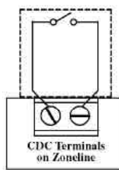
Typical Wiring
