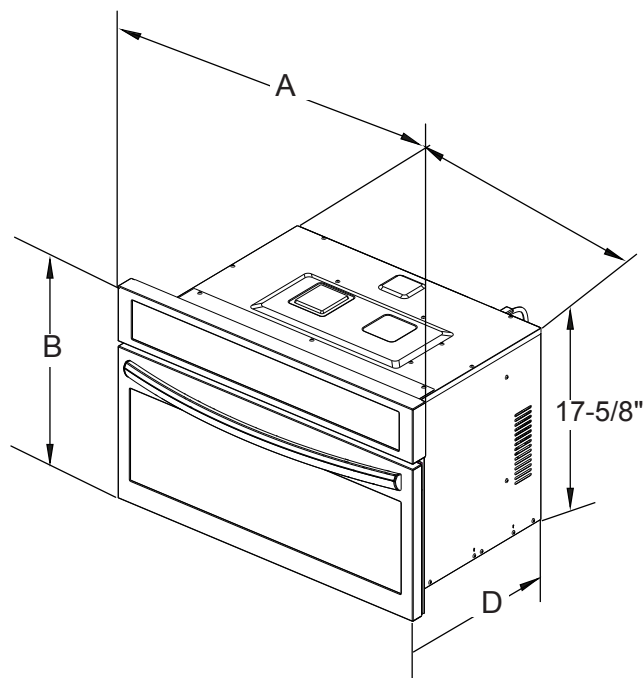
Figure 2: Microwave Only
