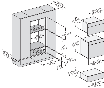
H 6x70 BM, ESW 6x85, DGC7x7x, H7x7x, Exx7x70 Fitting Combi, Installation drawing, Flush inset, NA
