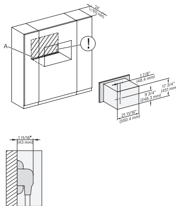
DGC7x7x(X), Installation, 30 Zoll, Proud, wide front, XL,
