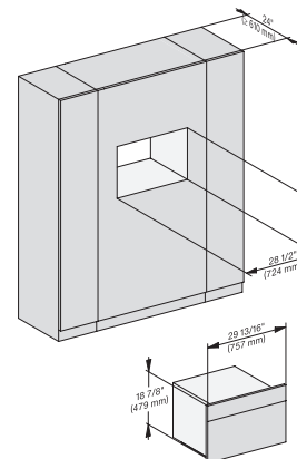
H 6x70 BM, DGC7x7x(X) fitting wide front, installation drawing, Proud, NA
