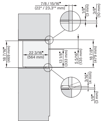
DGC7x7(X), side view, 30 Zoll, Flush inset, XL
