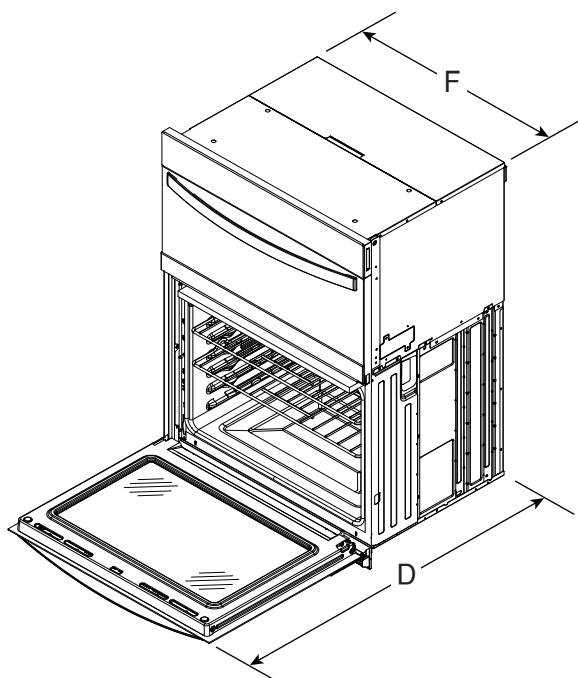
ANGLED VIEW
