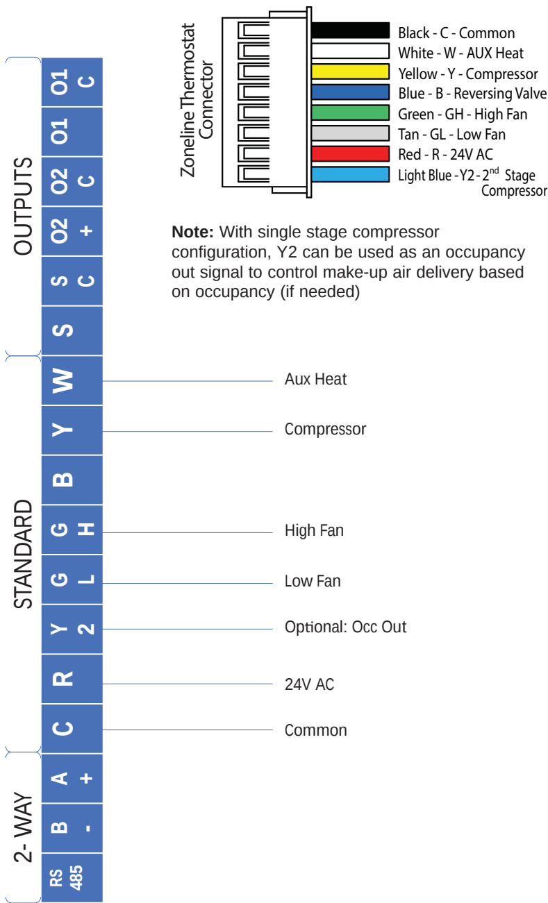
Diagram 5: Standard Communication Wiring (1 Heat / 1 Cool)
