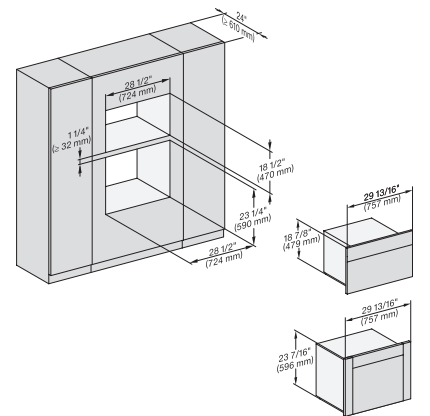
(H6560B, H6x60BP, DGC686xAM) + EBA680B; H6x70BM, DGC676x, NA7000, Fitting Combi wide front, Installation drawing, Proud
