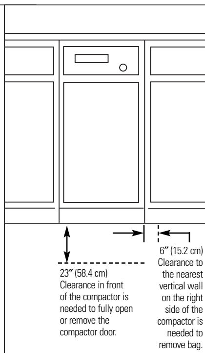
Clearance dimensions
