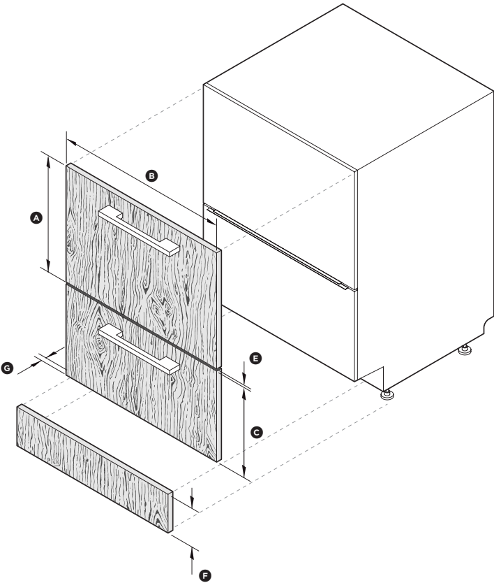
ISO VIEW
