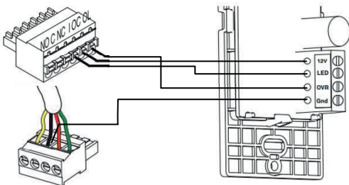
On-board terminal
