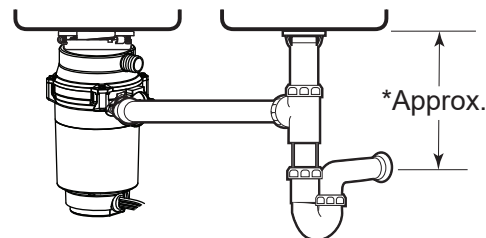
DOUBLE BOWL END OUTLET**
