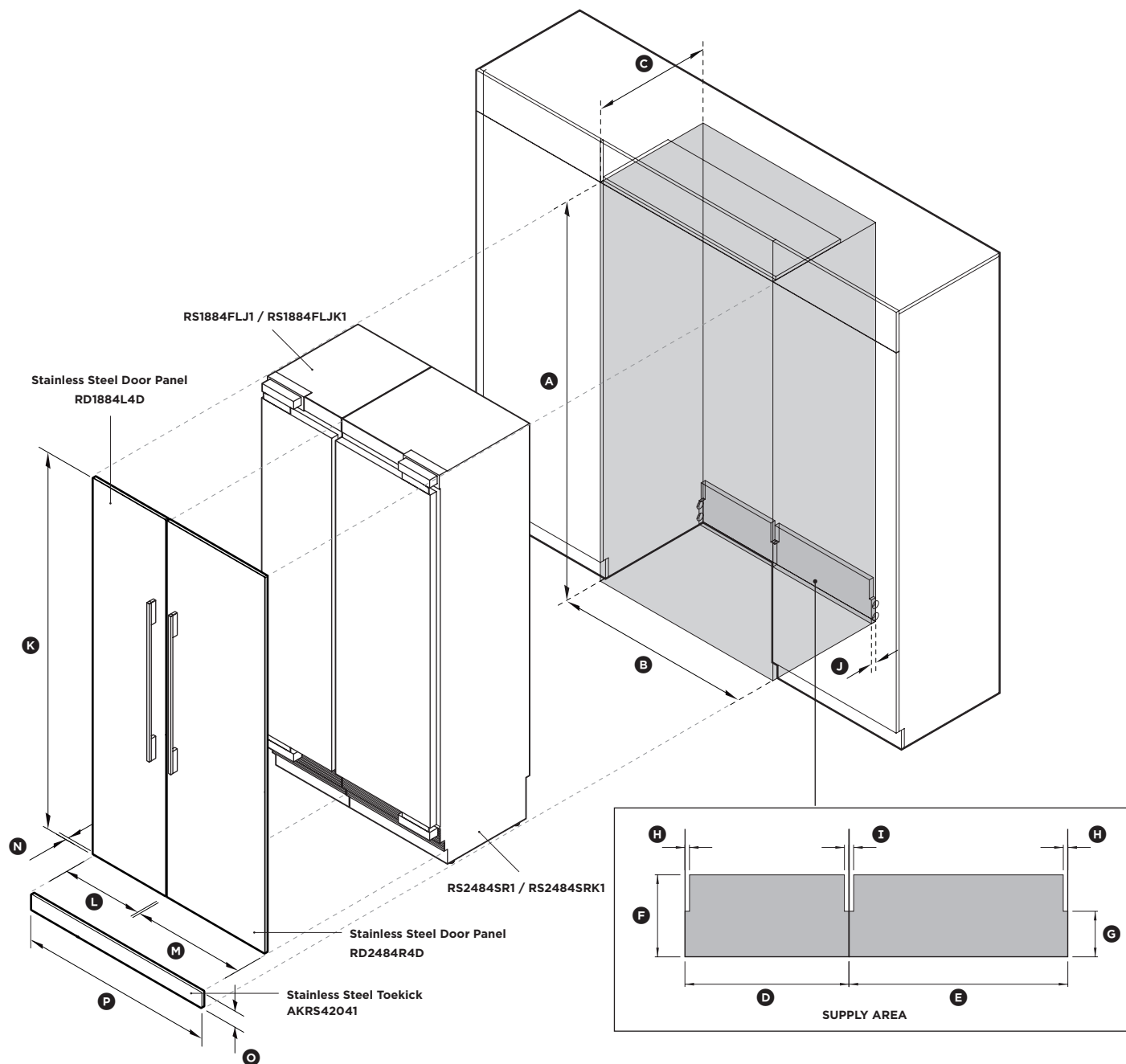
ISO VIEW OF 1067mm CAVITY (457mm + 610mm)
