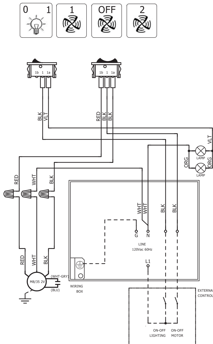
Wiring Diagram 991.0541.846
