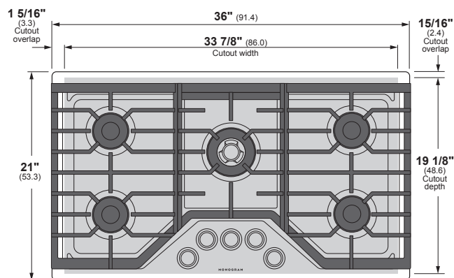
TOP VIEW (SHOWING CUTOUT OVERLAP)
