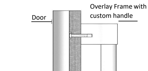
Round head screw hidden in a recession on the overlay.
