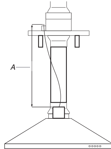
A. Distance between in-line smart kit and the range hood terminal box
