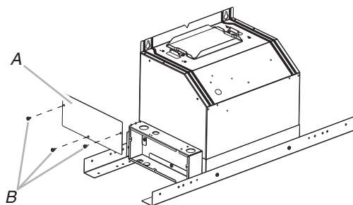
A. Terminal box cover B. Screws (3)
