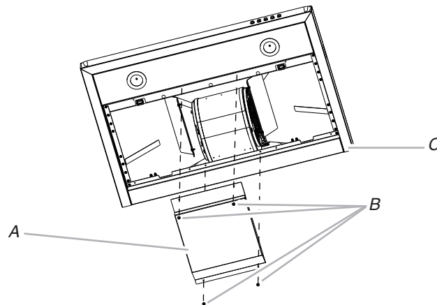
A. Blower motor cover plate B. Screws (4) C. Range hood
