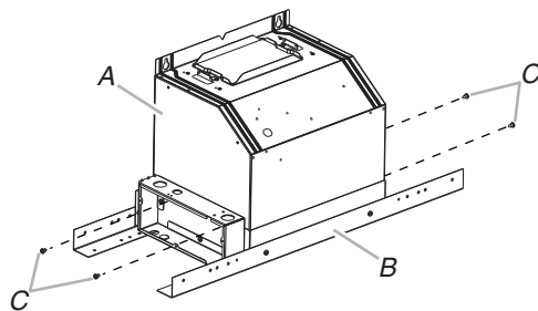
A. In-line housing B. In-line base C. Screws (4)
