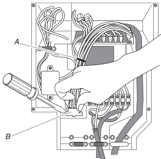
A. Wire tie B. 9-pin electrical connector (wires)
