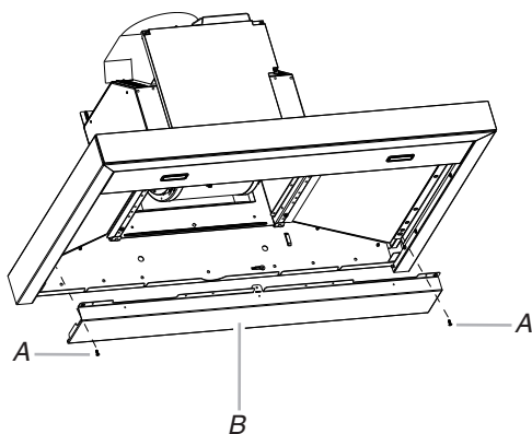
A. Bottom rear panel mounting screws B. Bottom rear panel
