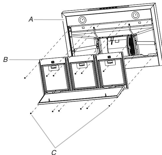
A. Range hood B. Filter retainer panel C. Screws (12)
