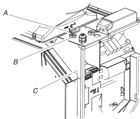
A. Electrical power wires (4) B. UL listed or CSA approved wire clamp C. Range hood electrical box
