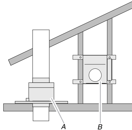
A. Mounted on top of ceiling joists (vertical duct) B. Mounted to cross-members tied to trusses (horizontal duct)
