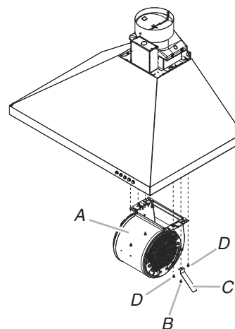
A. Blower motor B. Screws - insulation retainer (2) C. Insulation retainers (2) D. Screws - blower motor mounting (4)
