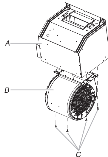
A. In-line housing B. Blower motor C. Screws (4)
