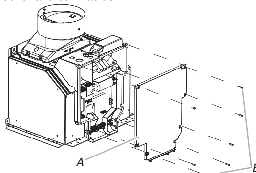
A. Plastic electrical box cover B. Screws (7)
