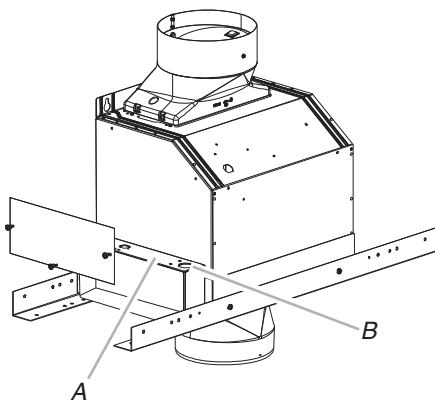
A. In-line smart kit terminal box B. Electrical knockouts
