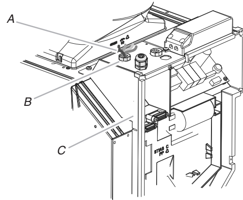
A. Electrical power wires (4) B. UL listed or CSA approved wire clamp C. Range hood electrical box
