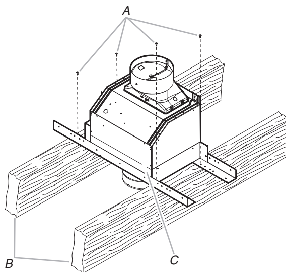
A. Mounting screws (4) B. Secure structure (joist, rafters or trusses) C. In-line smart assembly
