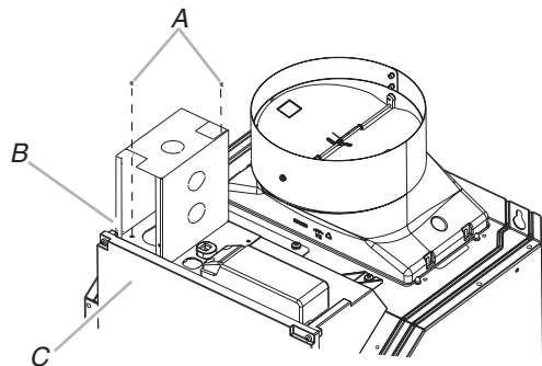
A. 3.5 x 6.5 mm screws (2) B. Metal terminal box C. Range hood electrical box
