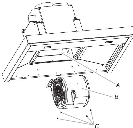
A. Range hood housing B. Blower motor C. Screws (4)
