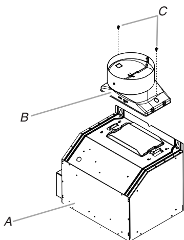
A. In-line housing B. Vent transition (with backdraft damper) C. 3.5 x 9.5 mm screws (2)
