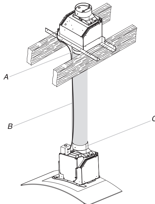
A. Vent transition - in-line smart kit (bottom) B. Vent system C. Vent transition - range hood
