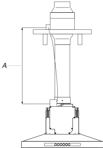
A. Distance between in-line smart kit and the range hood terminal box
