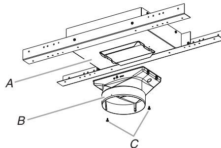
A. In-line base B. Vent transition (without backdraft damper) C. 3.5 x 9.5 mm screws (2)
