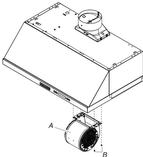
A. Blower motor B. Screws - blower motor mounting (4)
