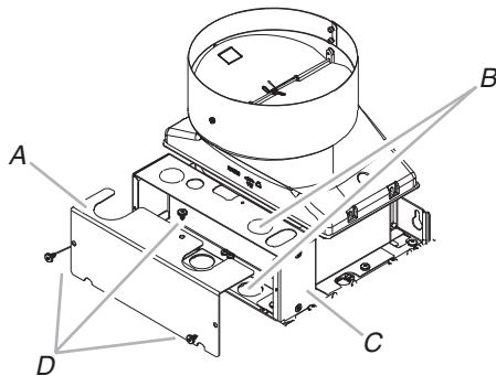
A. Range hood terminal box cover B. Electrical knockouts C. Range hood terminal box D. Screws (3)
