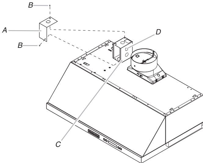
A. Terminal box cover B. Screws (2) C. Terminal box D. Electrical knockout
