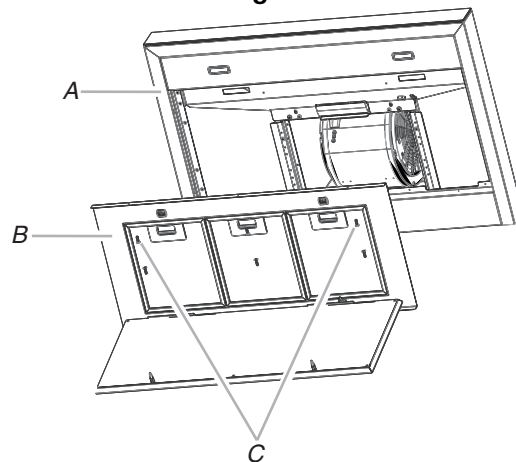
A. Range hood B. Filter retainer panel C. Screws (6)
