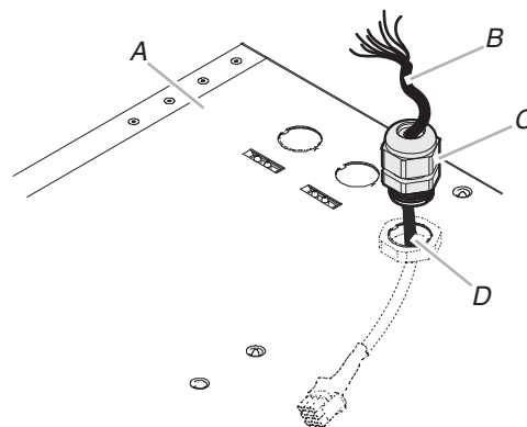
A. Range hood (top) B. 9-pin electrical connector (wires) C. UL listed or CSA approved plastic strain relief D. Electrical knockout
