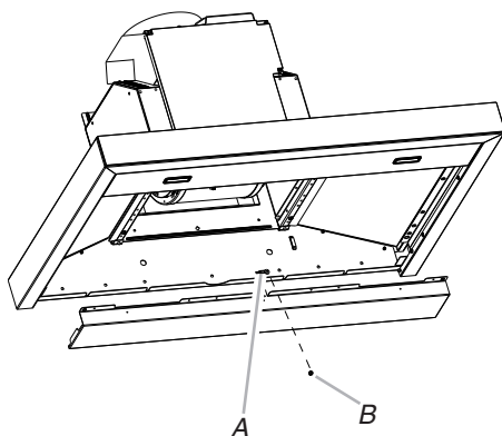
A. Temperature sensor B. Sensor mounting screw
