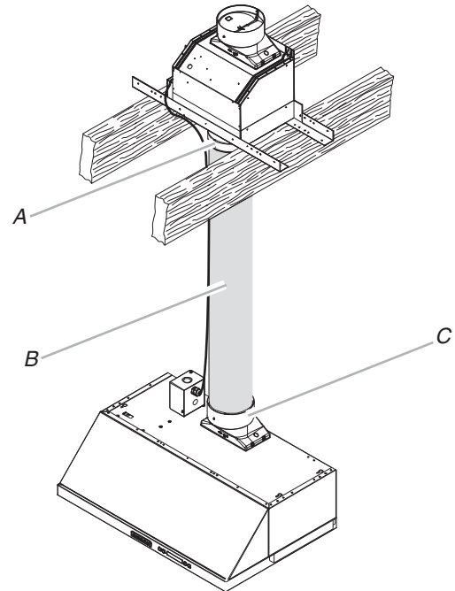
A. Vent transition - in-line smart kit (bottom) B. Vent system C. Vent transition - range hood
