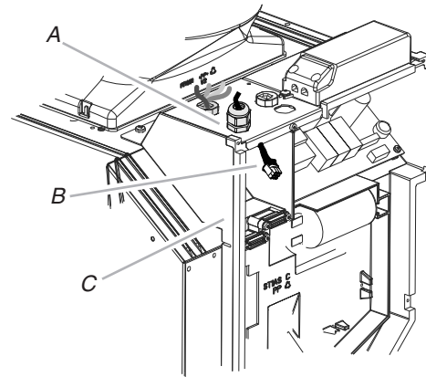
A. UL listed or CSA approved strain relief B. 9-pin pigtail electrical connector C. Range hood electrical box
