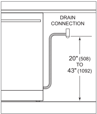
Drain connection
