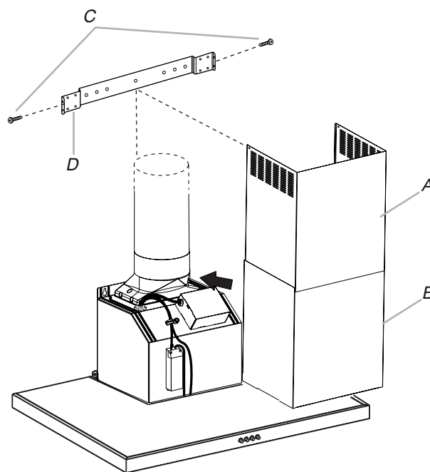
A. Upper vent cover B. Lower vent cover C. 4.2 x 8 mm screws D. Bracket
